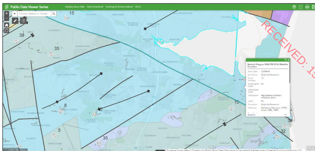
Figure 4.5. The underlying bedrock of the FCC Barrysparks Master Plan lands (“Argillaceous bioclastic limestone, shale” (Source: GSI))
