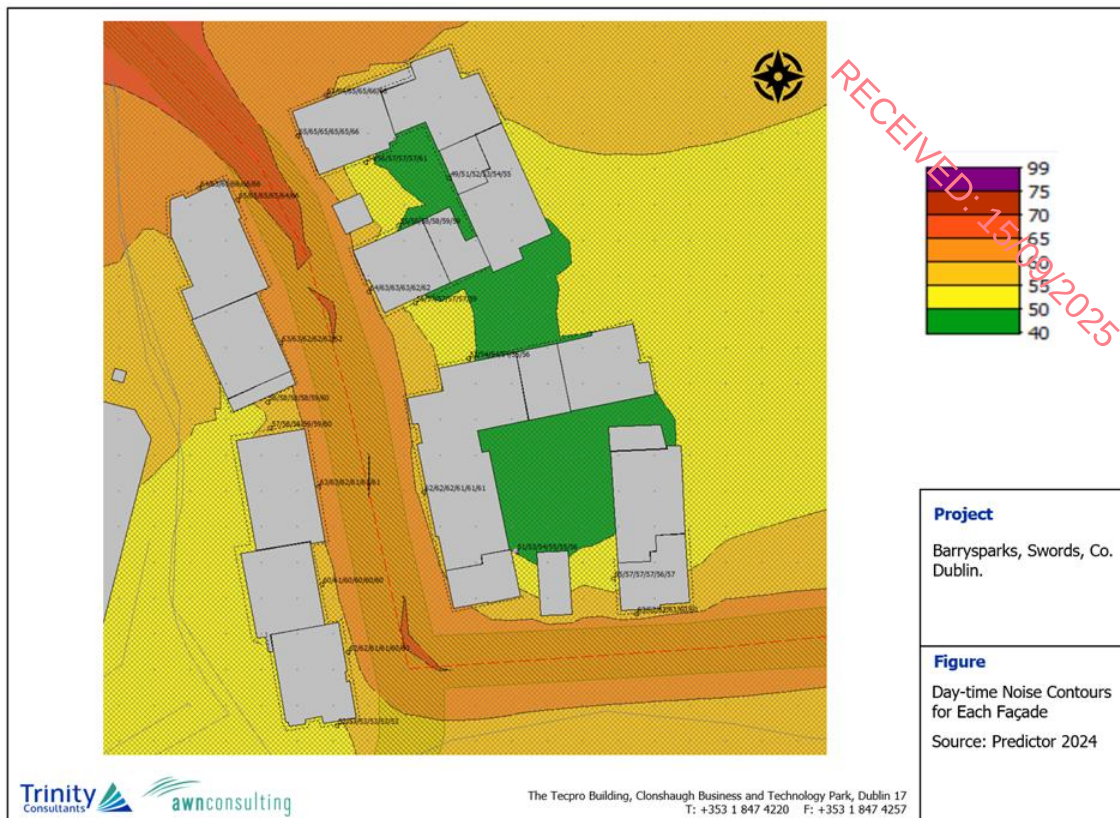
Fig 8.10: Day-time Noise Contours
