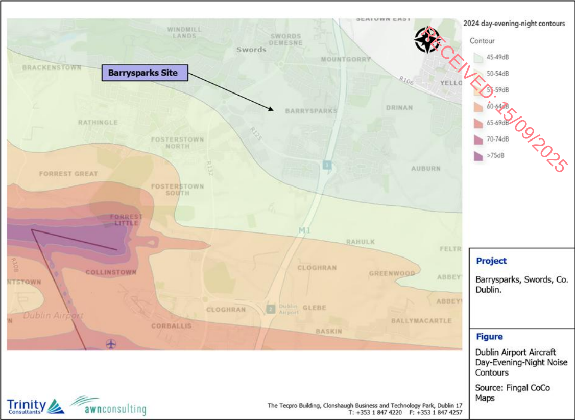
Fig. 8.5: L_{den} Dublin Airport Aircraft Noise Levels
