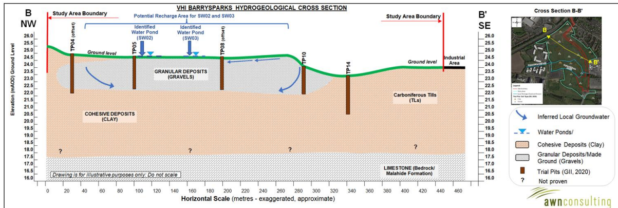
Figure 6.11 Hydrogeological cross section B-B'
