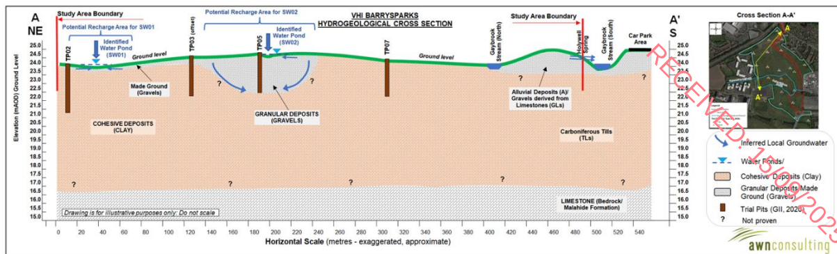
Figure 6.10 Hydrogeological cross section A-A'
