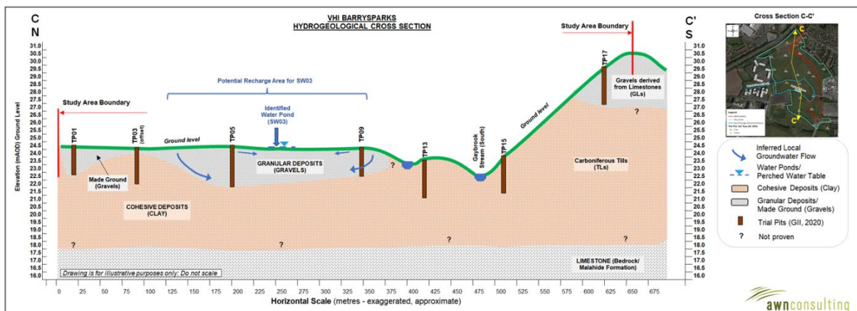
Figure 6.12 Hydrogeological cross section C-C'
