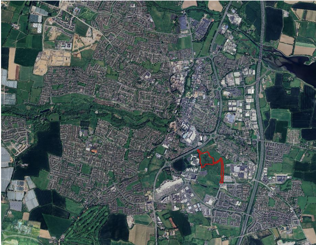
Figure 13.7: Site location in the mixed use character area between the R132 and the M1.
