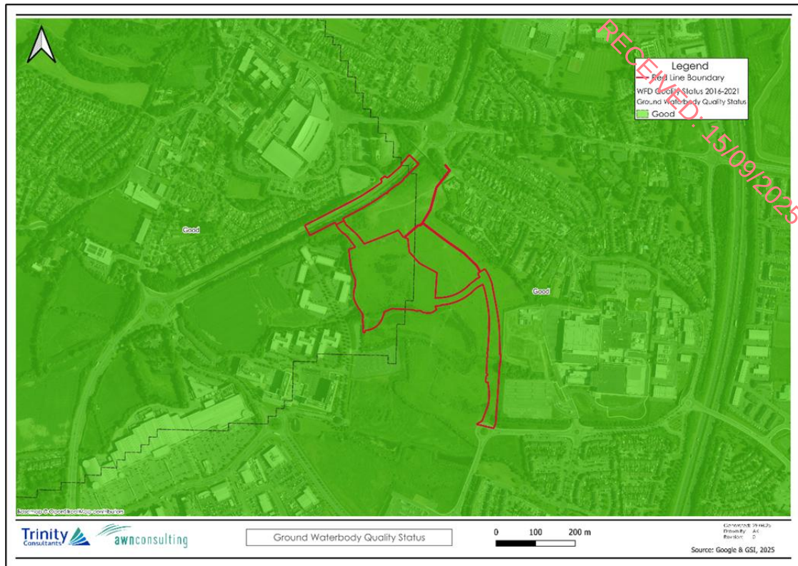
Figure 6.9 Ground Waterbody WFD Quality Status 2016-2021
