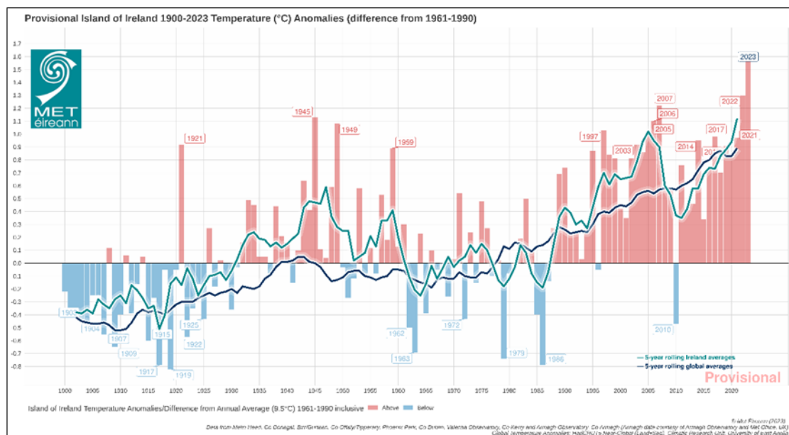
Figure 7.4 1900-2023 Temperature (°C) Temperature Anomalies(differences from 1961-1990)
