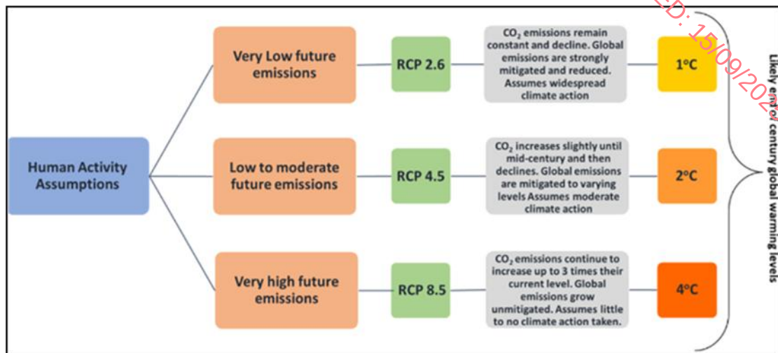
Figure 7.5 Representative Concentration Pathways associated emission levels
