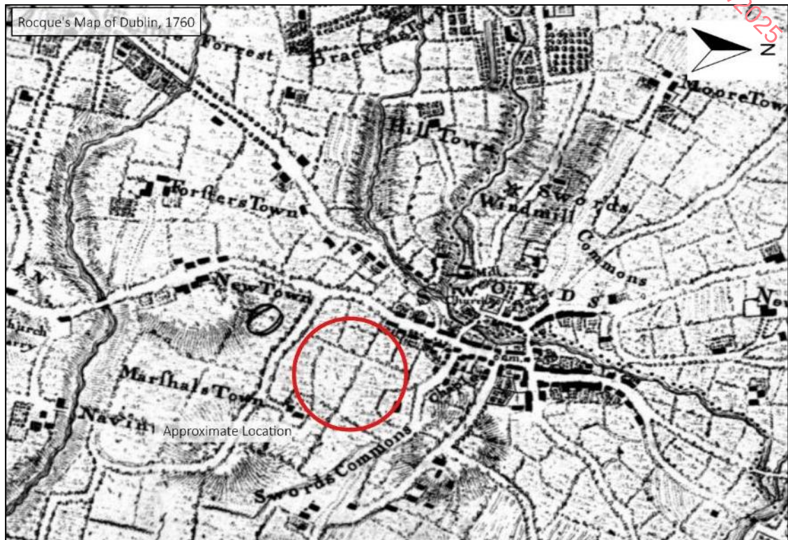
Figure 12.4: Extract from Rocque's map (1760)
