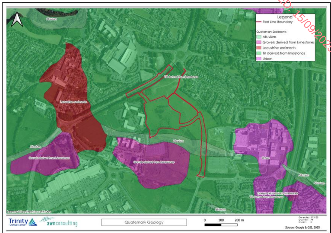
Figure 5.7 Quaternary Geology in the vicinity of the Proposed Development
