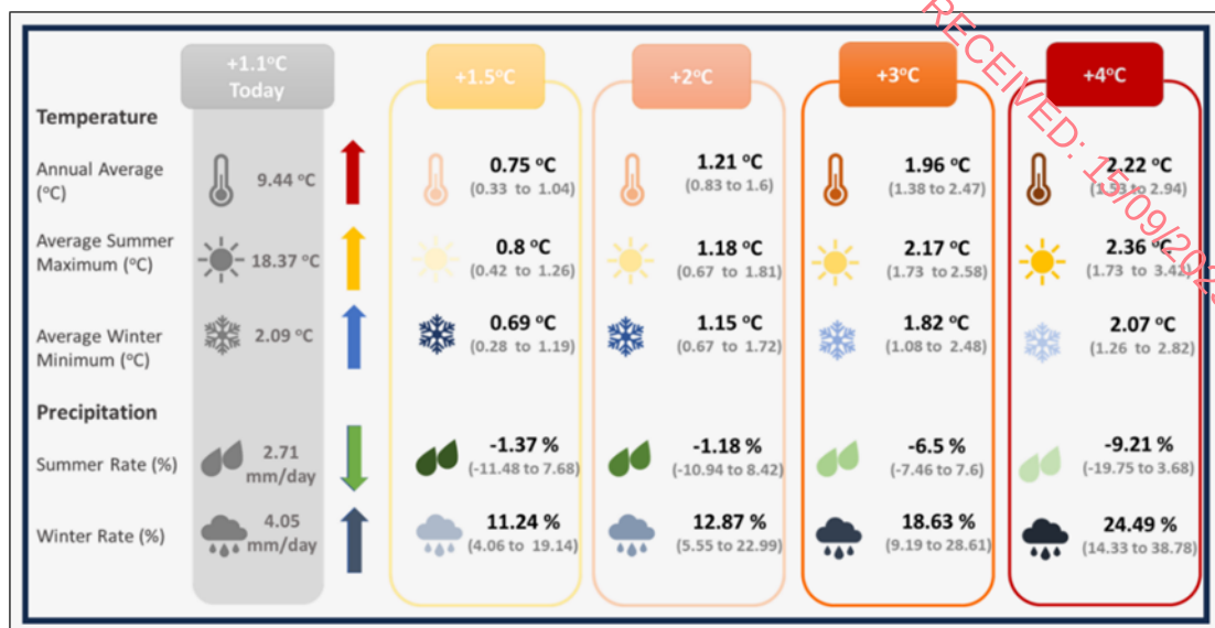
Figure 7.6 Change of climate variables for Ireland for different Global warming thresholds (Source: TRANSLATE Project Storymap, Met Éireann, 2023b)
