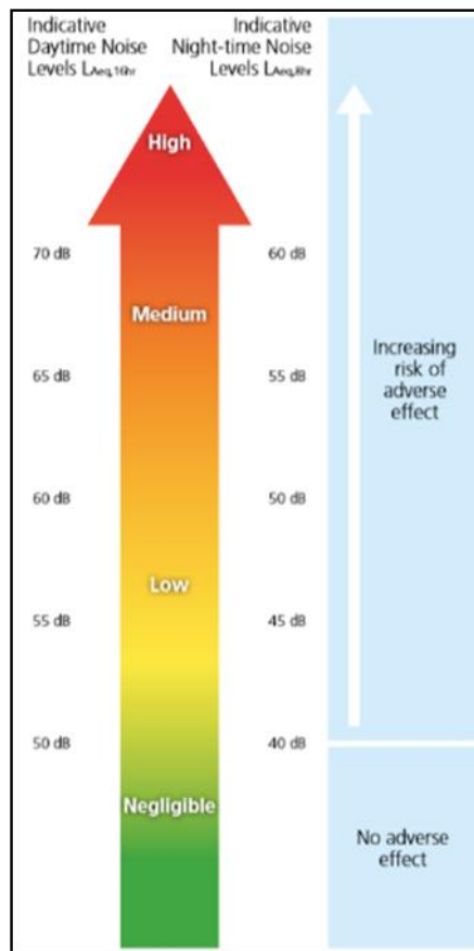
Fig 8.9: ProPG Stage 1 - Initial Noise Risk Assessment
